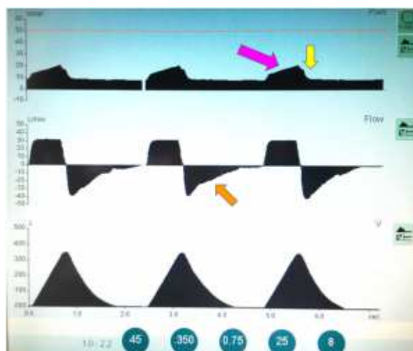
Figure 13: Waveforms in Volume Control Ventilation. Mechanical Ventilation module, ESICM Academy, 2018
