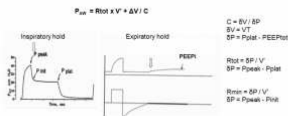
Figure 15: Measuring respiratory system resistance and compliance in volume control mode with constant flow. Mechanical Ventilation module, ESICM Academy, 2018
