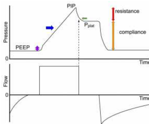
Figure 14: Waveform interpretation in Volume Control. Mechanical Ventilation module, ESICM Academy, 2018
